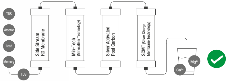
(ZX Double Protection Dual filter: Silver Activated Post Carbon + SCMT)
